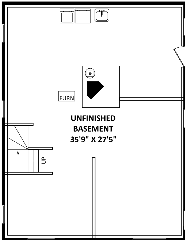
LOWER FLOOR: 1034 SQ. FT. (UNFINISHED)
