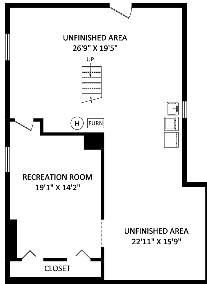
LOWER FLOOR: 1283 SQ. FT.
